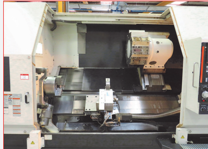
• Mazak Slanturn 50NR CNC Lathe with Mazatrol 640T CNC Control, 10-Position Turret, 2-Point Hydraulic Steady, Programmable Tailstock, 385mm 3-Jaw Hydraulic Chuck, Swarf Conveyor (05/2007)
