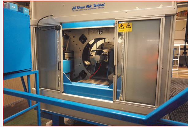
AB Korner MEK Verktast Borrautomat 4 Head Drilling and Turning Machine, Swarf Conveyor, 630mm 3 Jaw Chuck with various Face Plates, Knoll Coolant System (2003)
