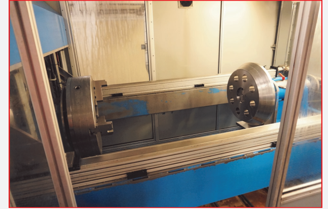
AB Korner MEK Verktast Borrautomat 4 Head Drilling and Turning Machine, Swarf Conveyor, 630mm 3 Jaw Chuck with various Face Plates, Knoll Coolant System (2003)
